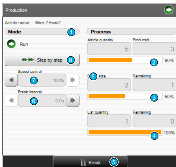
Fig. 20: Production screen, overview
