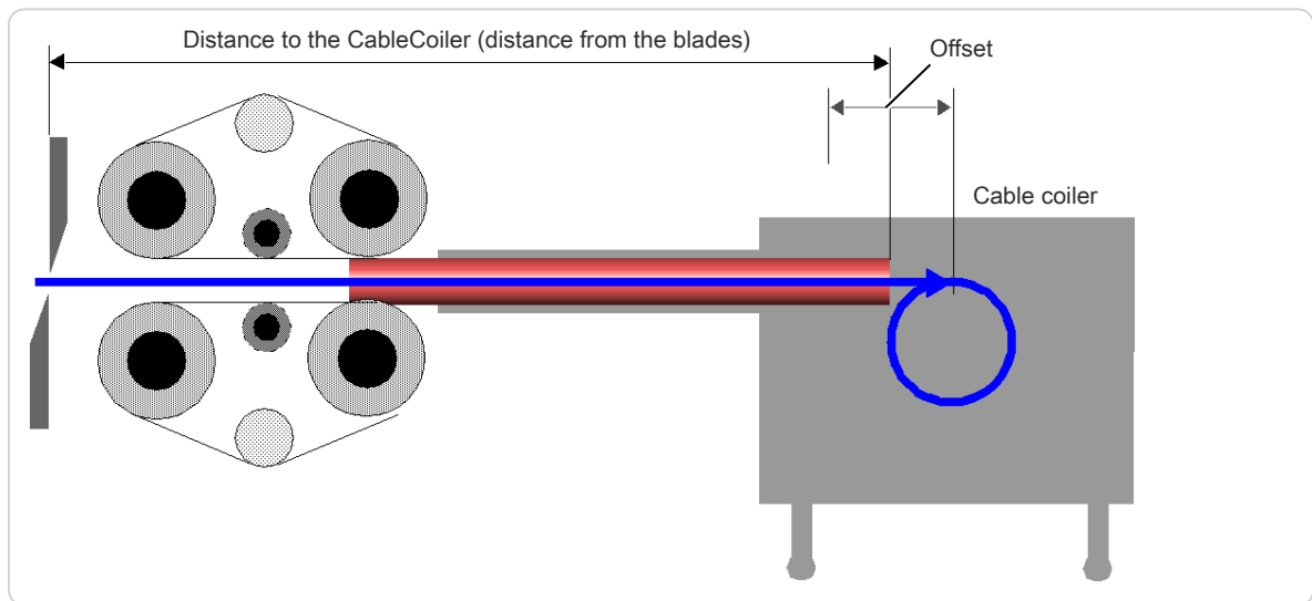
Fig. 26: Ejecting position cable coiler
