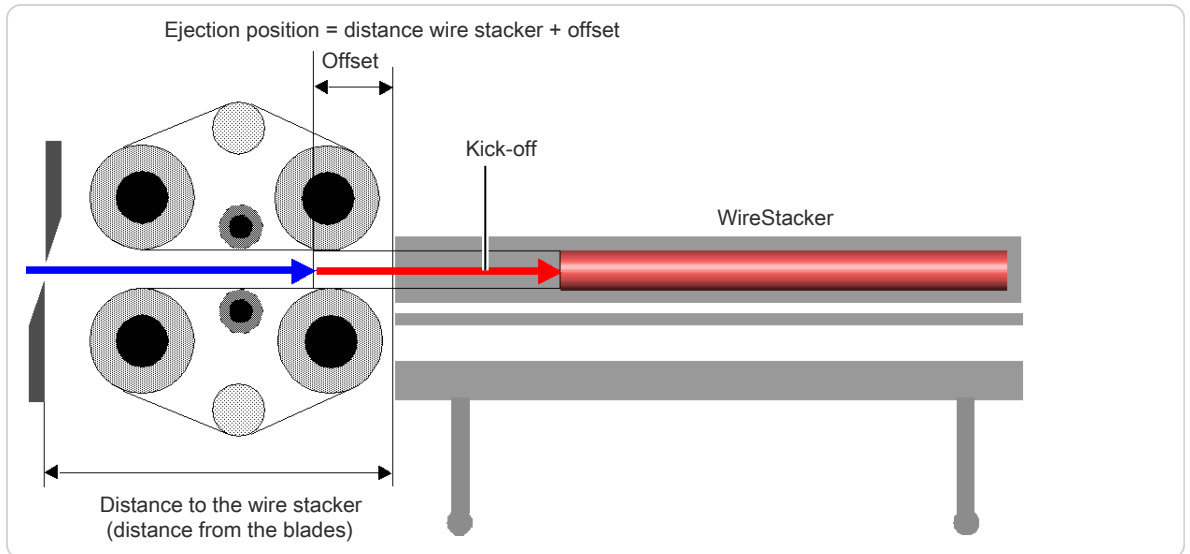
Fig. 25: Ejection with „Kick off“ activated
