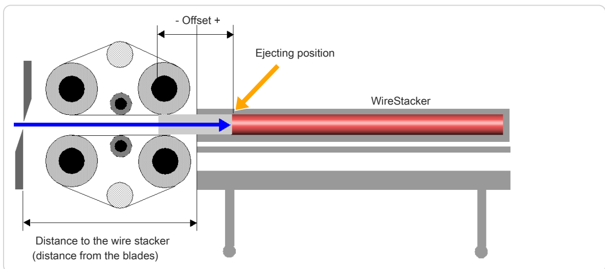
Fig. 24: Ejecting with offset
