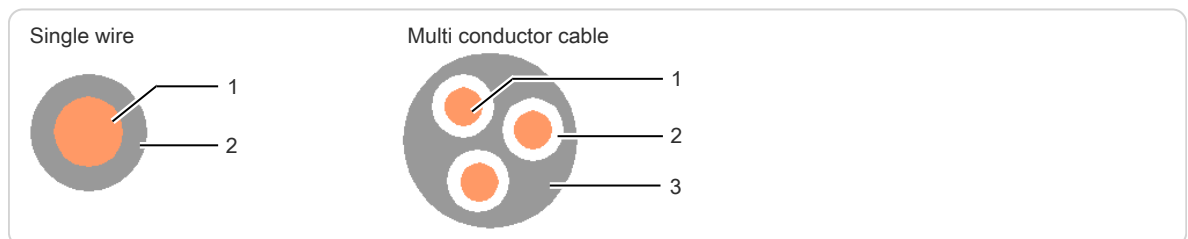
Fig. 14: Layer sectioning
