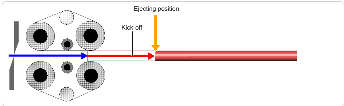
Fig. 23: Ejecting (kick-off)
