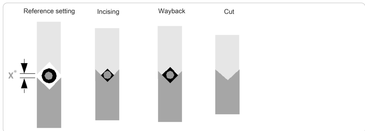
Fig. 9: Position of blades while feeding
